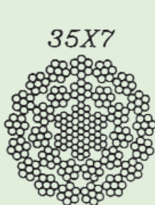
35X7 (1-6-6+W6-16)
